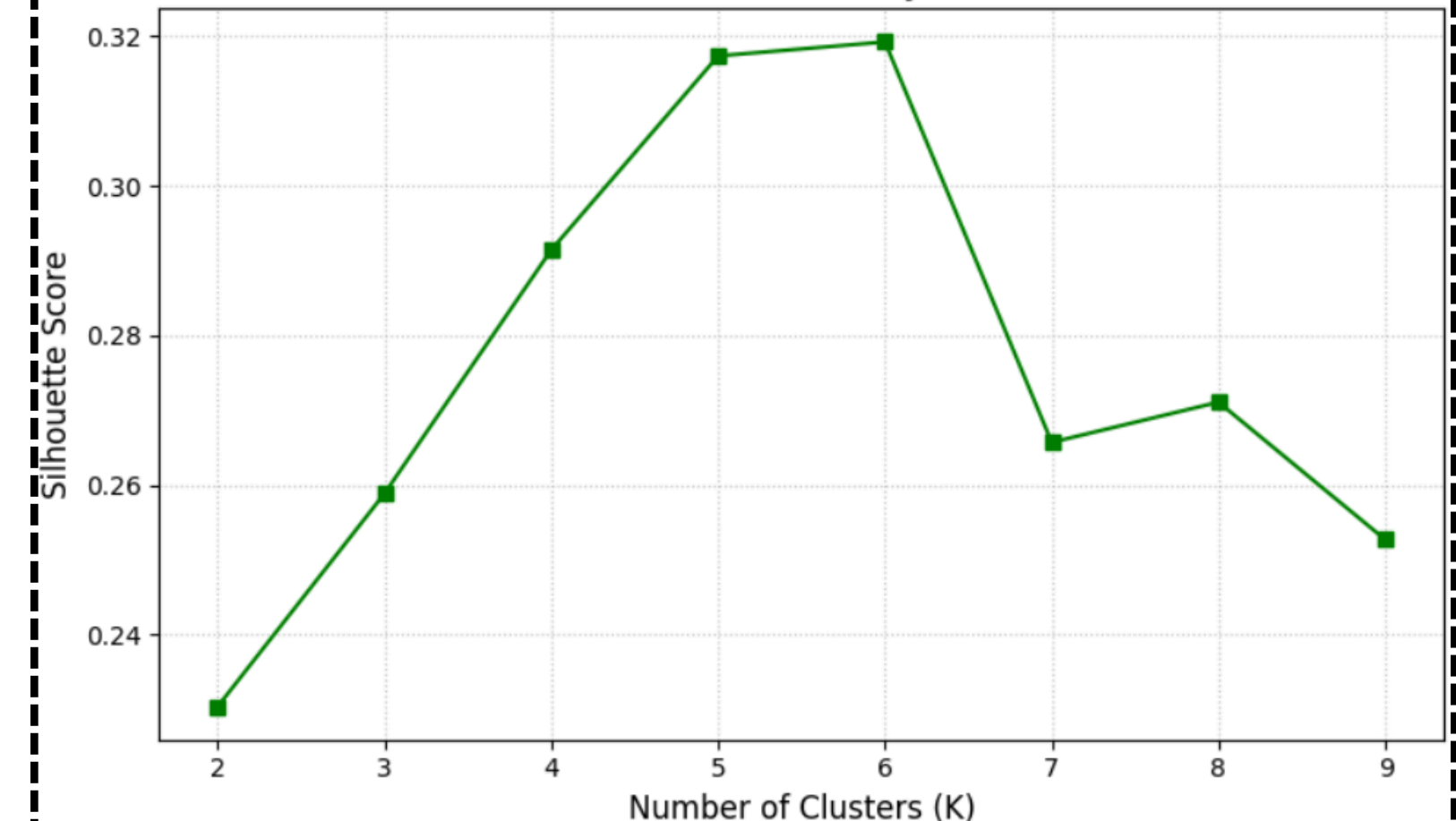
Silhouette Analysis
